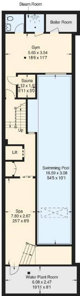
BASEMENT
